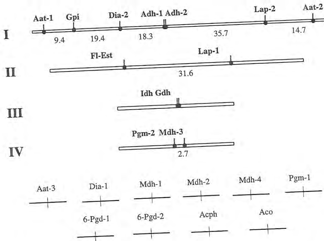
Fig. 10. Genetic map of Pinus mugo constructed on the basis of the results of isoenzyme electrophoresis. Distance in centiMorgans (cM).
