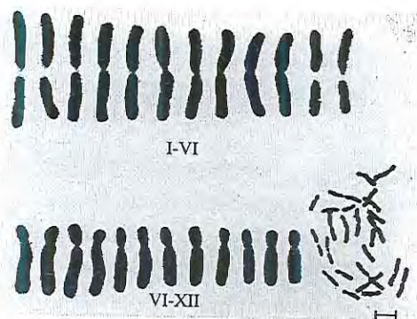
Fig. 1. Karyotype of Larix cajanderi Mayr. I-VI, VII-XII are the chromosome numbers. Bar = 10 mm.
