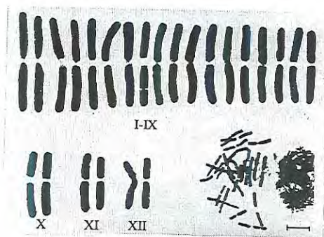
Fig. 3. Karyotype of Pinus densiflora Siebold et Zucc. I-IX, X, XI, XII are the chromosome numbers. Bar = 10 mm.
