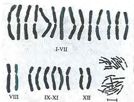
Fig. 5. Karyotype of Abies sibirica Ledeb. I-VII, VIII, IX-XI, XII are the chromosome numbers. Bar = 10 mm.
