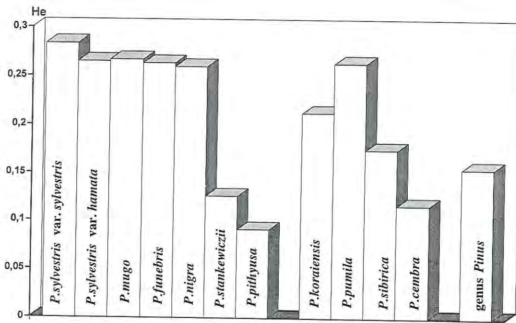
Fig. 3. Levels of genetic variability based on expected heterozygosity ( H_e ) values in pine species occurring in the territory of the former USSR. The average data on the genus Pinus are taken from the current study, from Goncharenko et al. (1993c) as well as from studies of Gibson and Hamrick 1991, Mosseler et al. 1991, Boscherini et al. 1994, Goncharenko et al. 1994, Kim et al. 1994, Edwards and Hamrick 1995.
